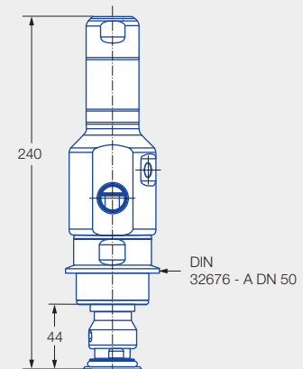
Tri-Clamp-Anschluss 5P9
