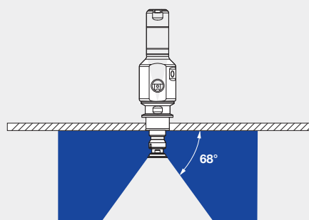
Tri-Clamp-Anschluss 5P8
