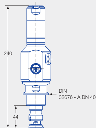
Tri-Clamp-Anschluss 5P8
