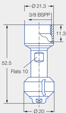
Female thread
