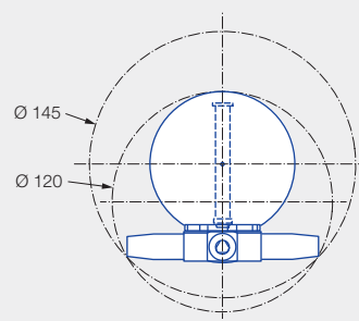
Insertion diameter and interference circle diameter of the slip-on connection
