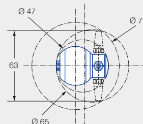
Insertion diameter and interference circle diameter
