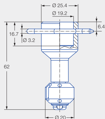
Dimension of the slip-on connection according to ASME-BPE (OD tube)
