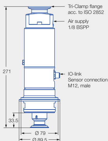
Tri-Clamp flange
