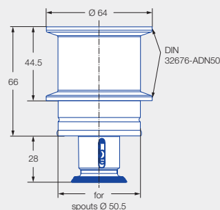
Tri-Clamp connection 2
