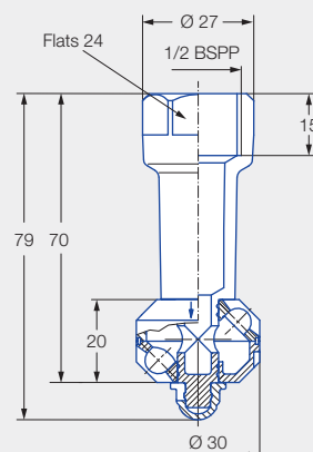
Female thread
